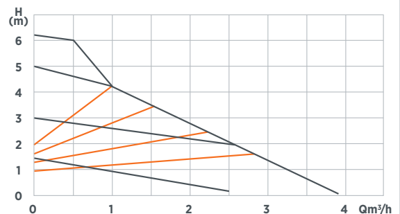
Characteristic WITA go.future light 60
