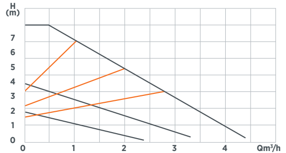
Characteristic WITA Delta Plus UE 70A
