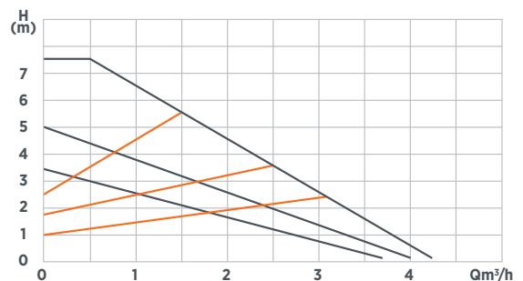
Characteristic WITA Delta Plus UE 75A
