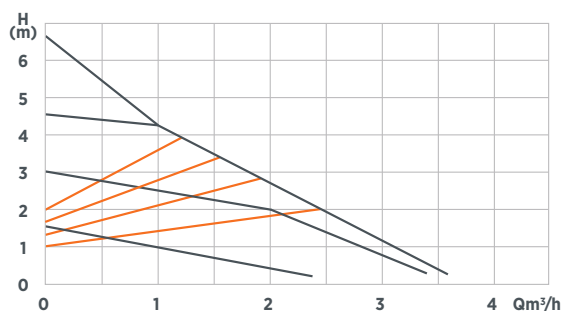
Characteristic WITA HE go.future 60 light
