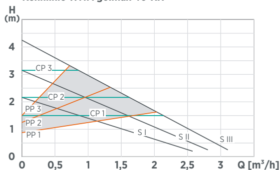
Kennlinie WITA go.max 40-XX
