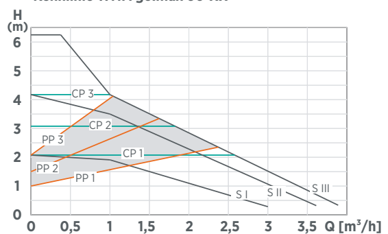
Kennlinie WITA go.max 60-XX
