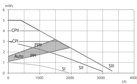
Kennlinie WITA HE+ go.future | 50-xx
