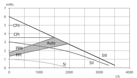
Kennlinie WITA HE+ go.future | 60-xx
