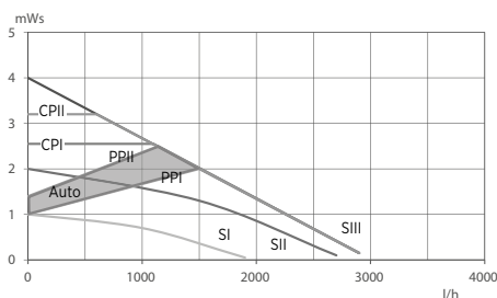
Kennlinie WITA HE+ go.future | 40-xx
