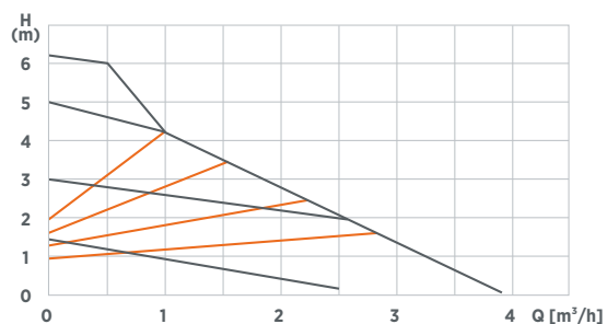
Kennlinie WITA Delta HE light 55
