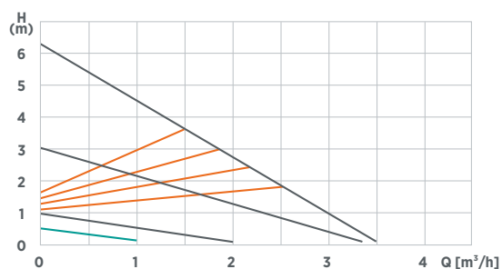
Kennlinie WITA Delta HE 55 LED
