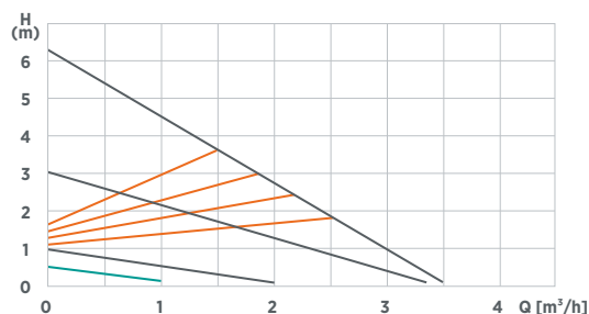
Kennlinie WITA Delta HE 55 LCD
