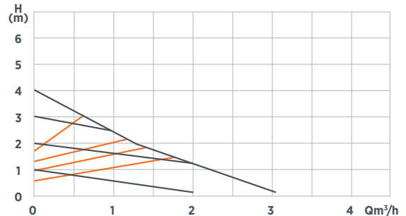
Kennlinie WITA go.future light 40
