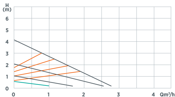
Kennlinie WITA go.future 40 LED
