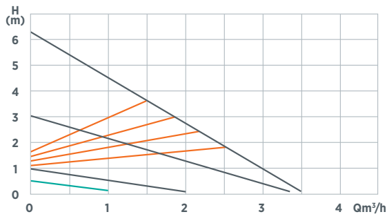
Kennlinie WITA go.future 60 LED
